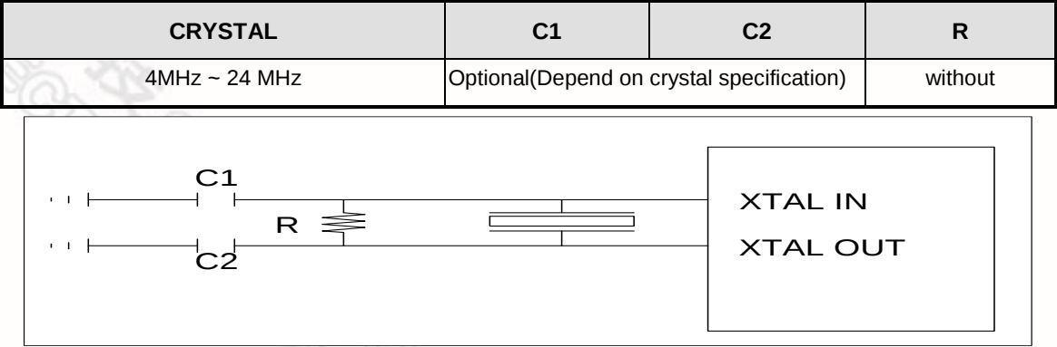
Figure 9-1 Typical Crystal Application Circuit
